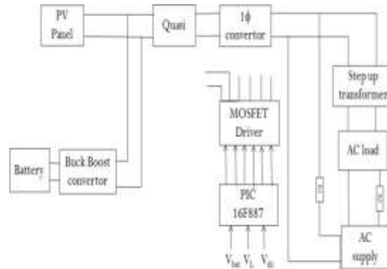
Fig.6 Block Diagram
