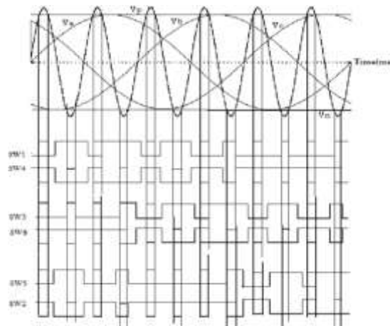
Fig.5. Schematic of Sine PWM
