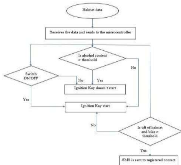
Fig.14. Flowchart of Bike Section
