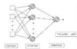
Fig. 1. Neural Network
