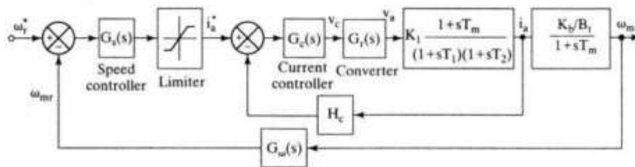
Fig.1.Block diagram of Speed control of DC motor
