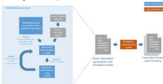
Figure 8: Proposed simulation flow for switching power converters
