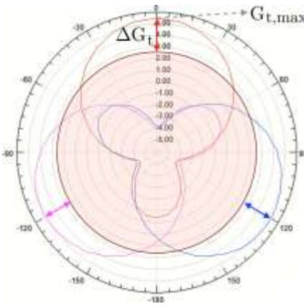
Figure6. ThreeALR-A0501antennas radiation plot.
