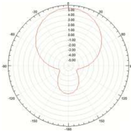
Figure5. ALR-A0501antenna radiation plot.
