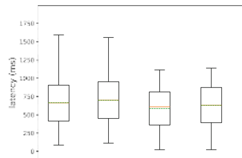
Fig. 10: The average end-to-end packet transmission latency of the four sensor nodes integrating the gas sensor arrays. The statistics were generated based on the reception of 2000 packets. The two left bars correspond to the nodes which were 4-hop away from the base station, whereas the two right bars correspond to the nodes which were 2-hop away from the base station.
