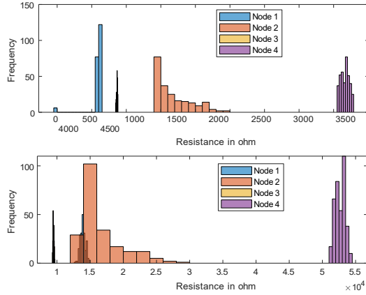
Fig. 6: Comparison of the histograms of the min and max operations. Only Node 2 was exposed to ammonia.
