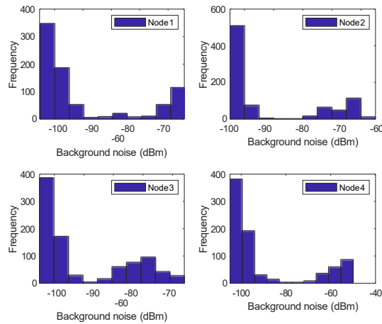
Fig.7: The statistics of the background noise as perceived by the four sensor nodes integrating the arrays of gas sensors (Channel25).
