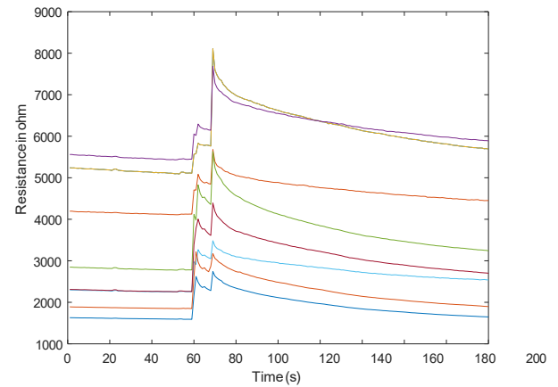
Fig.4: The difference in the raw values of nine arbitrarily selected sensors of an array in the presence of ammonia (right).
