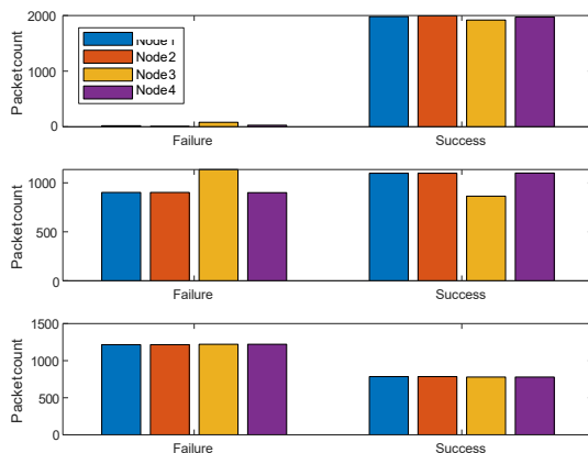
Fig.8: Comparison of the total number of packets transmitted and the total number of packets received by the base station. The transmitters were the four nodes integrating the ammonia sensor arrays. The two nodes farthest away from the base station were each four-hop away and the two nodes nearest to the base station were each two-hop away. Top: Channel 25. Middle: Channel 26. Bottom: Channel124.
